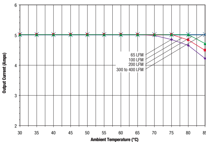
Maximum Current Temperature Derating @ sea level ( V_{IN} = 48V , transverse airflow, no baseplate)
